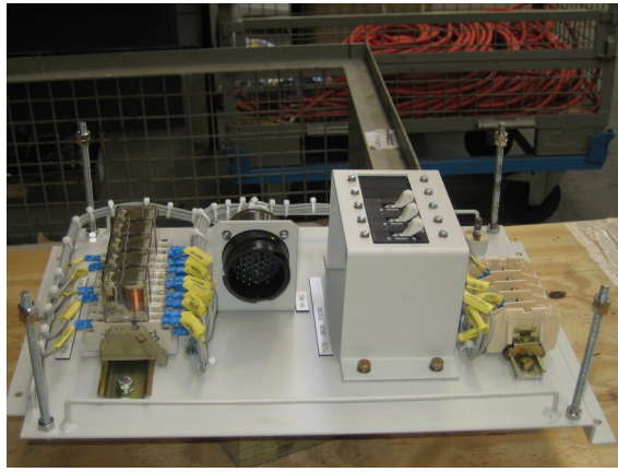
MCB Panel
