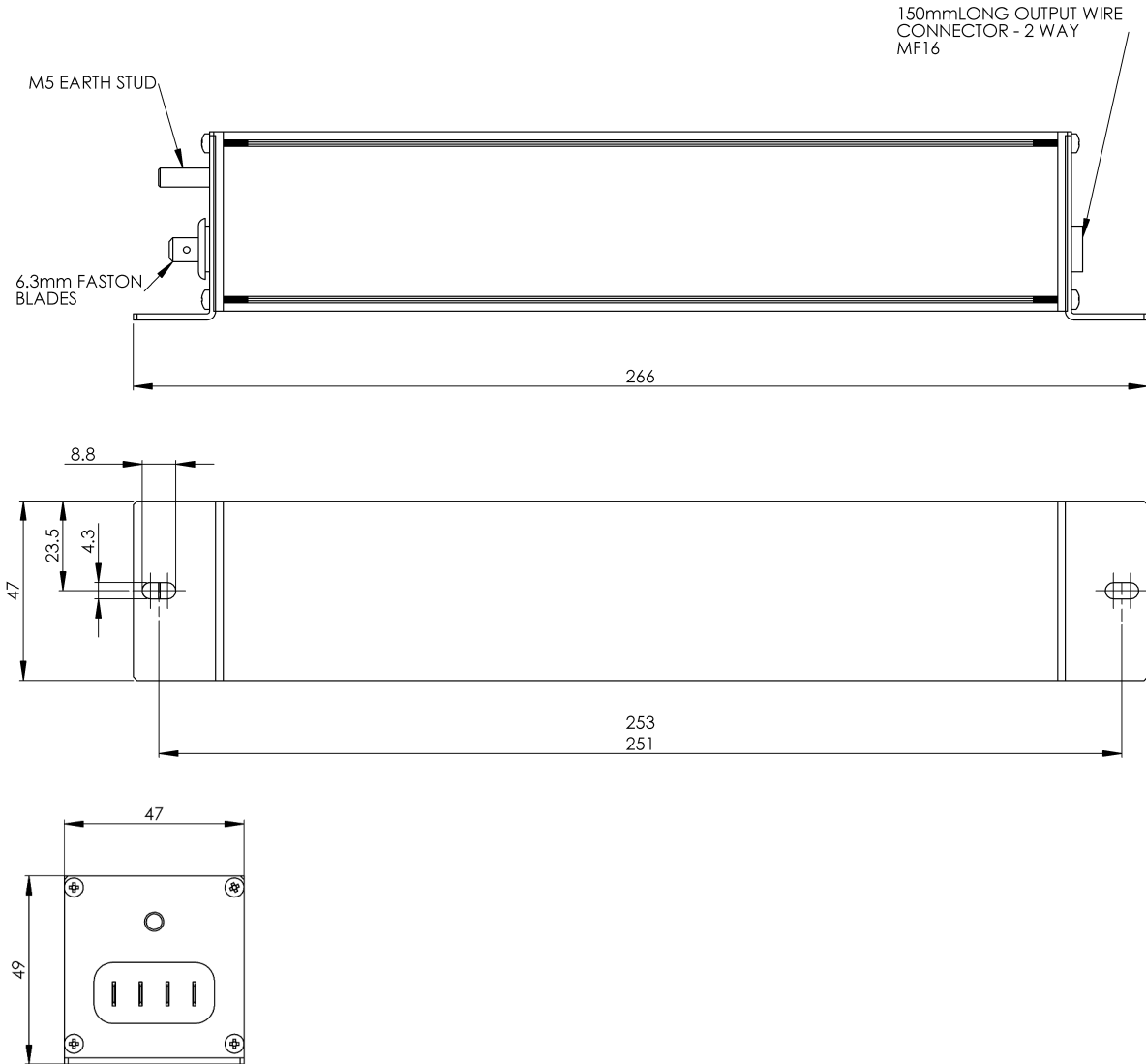
Figure 1 - Enclosure Details for 67125 LED PSU 0.25" Faston Blades & Entrelec MF16 Connectors
