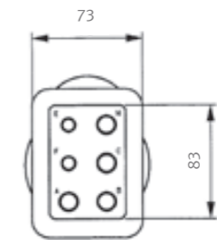
Type 14 Plug
