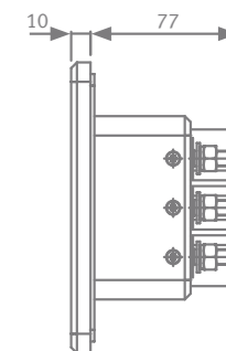
All dimensions in mm
